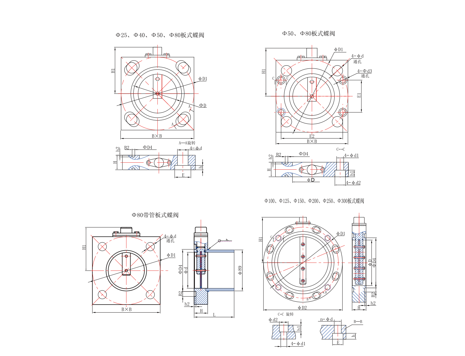
BDB 系列板式蝶阀尺寸表 Specification of BDB series of plate type butterfly valve
