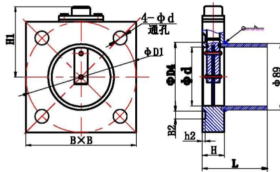
Plate type butterfly valve with pipe \Phi 80
