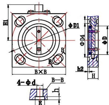
Φ50、Φ80 Vacuum valve connect to cover
