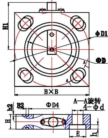
\Phi 50 、 \Phi 80 Plate valve with connection on tank cover \Phi 50 、 \Phi 80 Plate Valve with connection to relay
