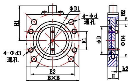
Φ50、Φ80 Vacuum valve to Relay
