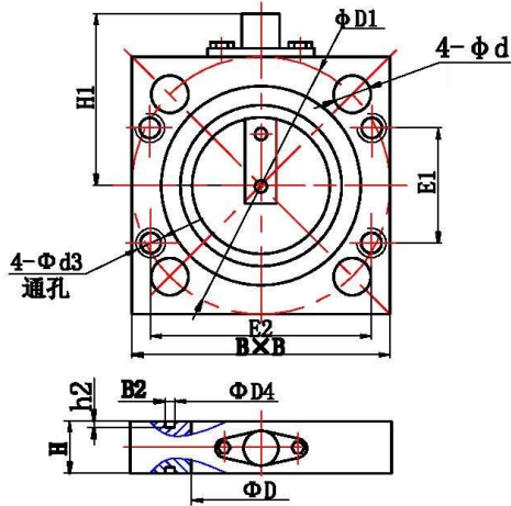
\Phi 50 、 \Phi 80 Plate valve with connection on tank cover \Phi 50 、 \Phi 80 Plate Valve with connection to relay
