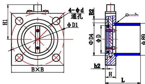
Φ80 Vacuum valve with pipe
